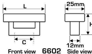
Front view 6602
