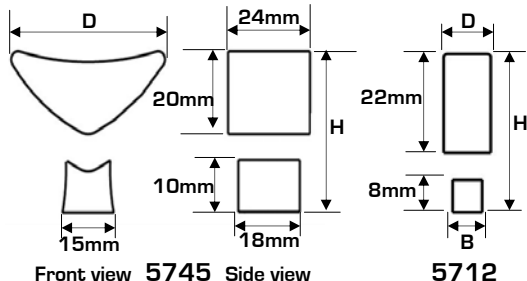
Front view 5745 Side view
