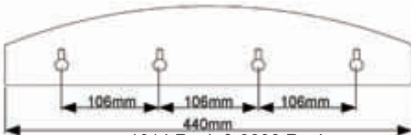
1014 Rack & 9338 Rack
