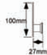
9338 side view
